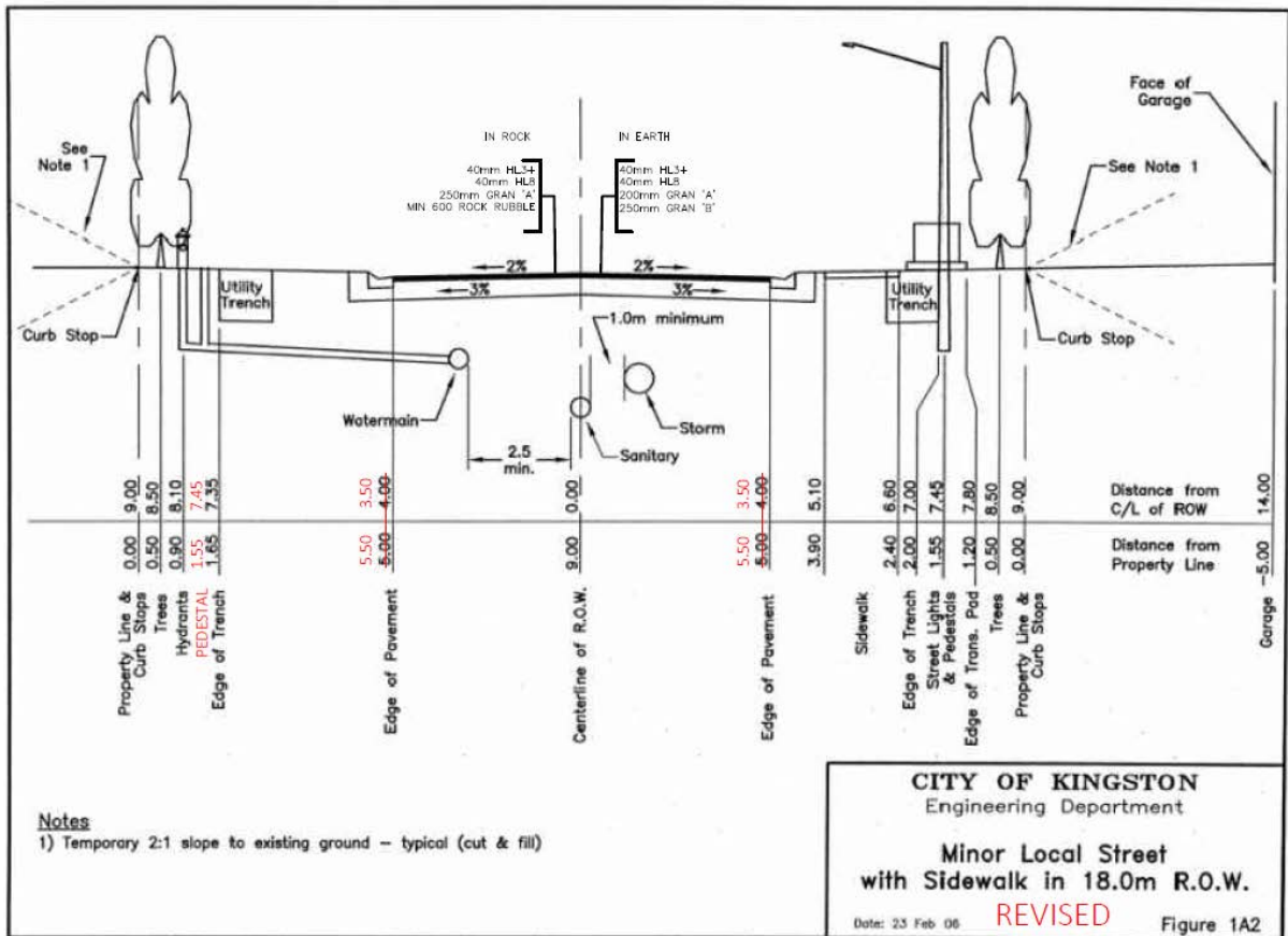
Figure 1A2 Minor Local Street – 18m Right of Way (with Sidewalk)
